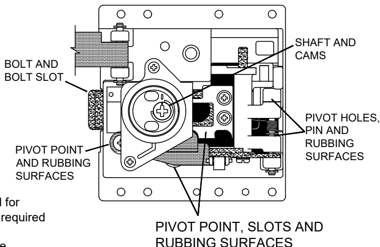
Lubrication Diagram
