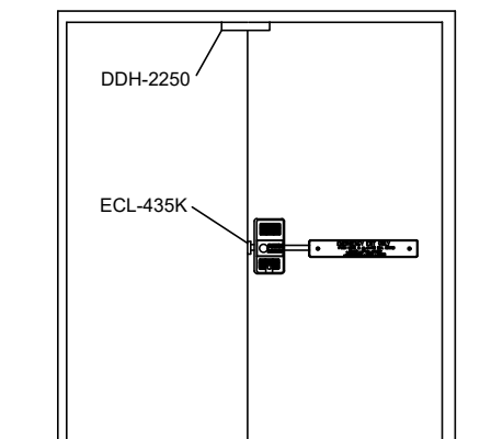
DOUBLE DOORS
