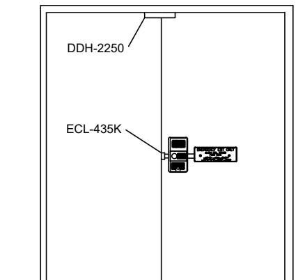
DOUBLE DOORS
