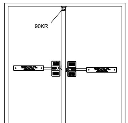
DOUBLE DOORS WITH REMOVABLE MULLION
