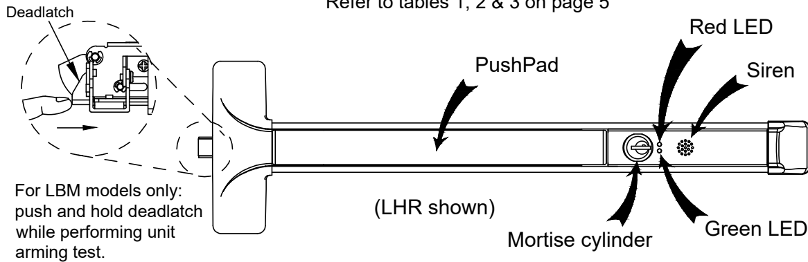
Figure 1 Device features.
