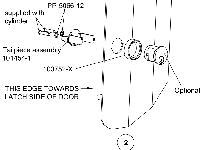
Install Tailpiece Assembly
