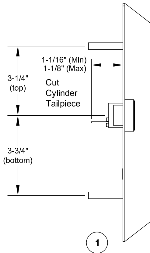
Rim Cylinder Preparation
